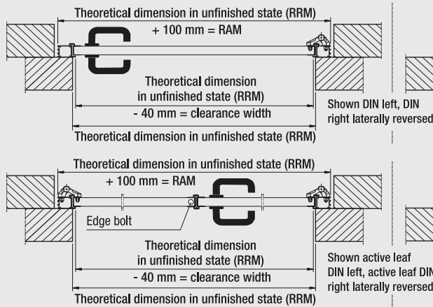
Installation behind the soffit, only inward opening
